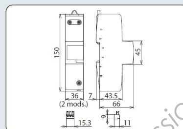
Dimensions DBM 1 440 FM
